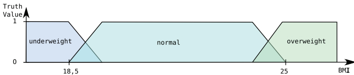
Figure 2: Three fuzzy sets
